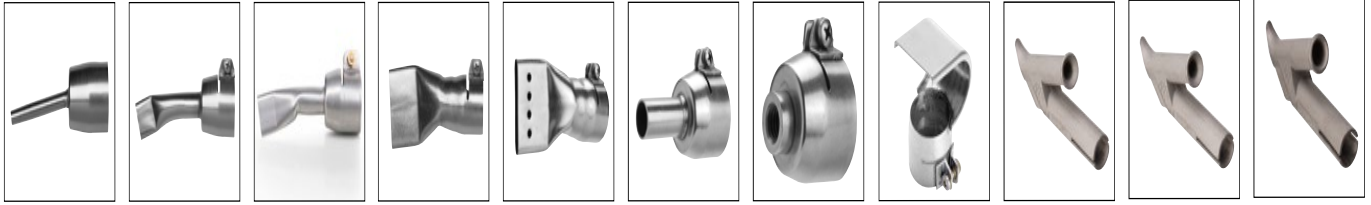
Item No. 4000 Round nozzle, 5 mm Item No. 4002 Nozzle, 20 mm flat Item No. 4002.15 Nozzle 20 mm flat, 15° angled, for roofing Item No. 4003 Nozzle, 40 mm flat Item No. 4004 Nozzle 40 mm flat, perforated Item No. 4005 Shrink nozzle 15 mm, round Item No. 4007 Adapter with thread M 10 Item No. 5016 Shrink reflector Item No. 5010 Speed welding nozzle for nozzle item No. 4000, 3 mm, round Item No. 5011 Speed welding nozzle for nozzle item No. 4000, 4 mm, round Item No. 5012 Speed welding nozzle for nozzle item No. 4000, 5 mm,
